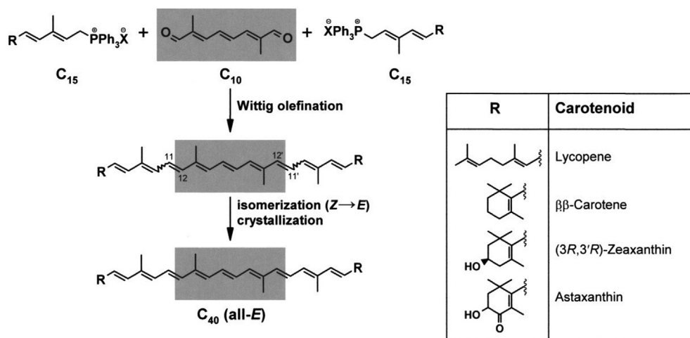
Fig. 7. Industrial synthesis of commercial carotenoids.
