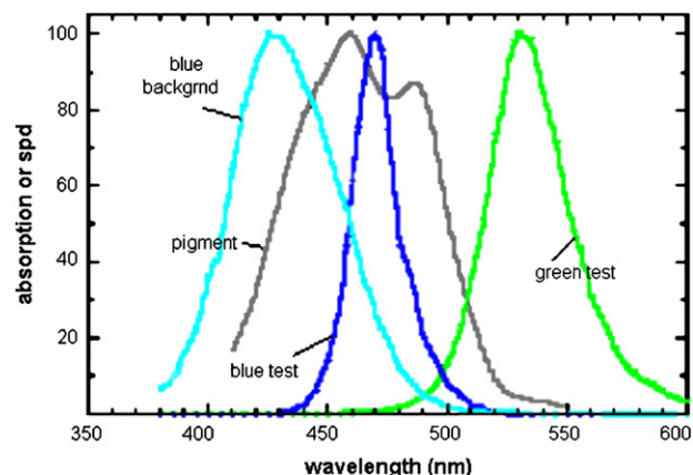
Fig. 1. Normalised spectral power distribution of the LEDs used in the maculometer together with the normalised spectrum of MP.
